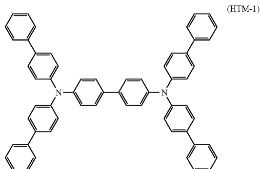
(HTM-1)
