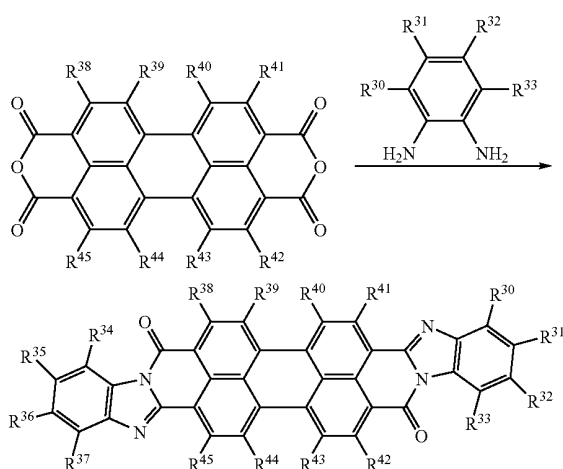
(Synthesis scheme 4)
