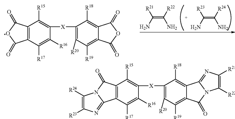
(Synthesis scheme 3)
