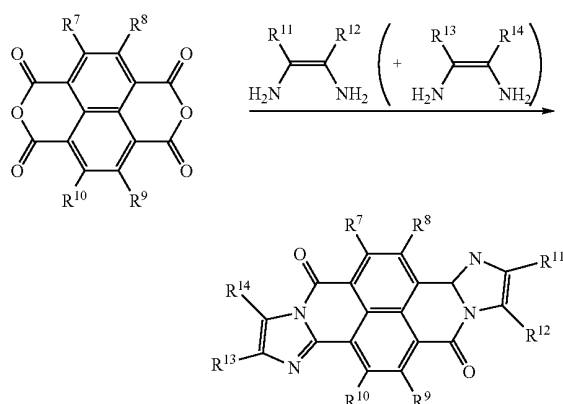
(Synthesis scheme 2)
